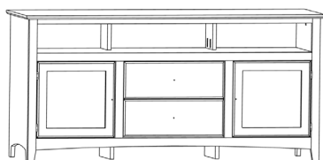
30" High 61"W Console 6861 30"H x 61¾"W x 18"D 61"W Console - Flush 6861F 30"H x 59¾"W x 18"D
